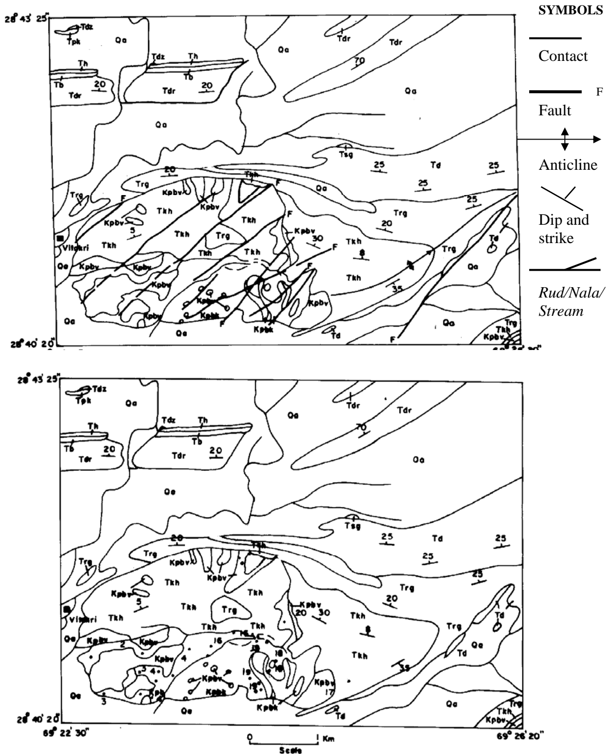
Fig. 2. Upper, Geological map of Vitakri area. Lower, Dinosaur localities and fossil sites (dots) map of Vitakri area. Abbreviation; Qa, Alluvium; Tdz, Drazinda F. Tpk, Pirkoh F. Tdm, Domanda F. Thr, Habib Rahi F. Tb, Baska F. Tdr, Drug F. Tsg, Shaheed Ghat F. Td, Dungan F. Trg, Rakhi Gaj F. Tkh, Khadro F. Kpbv, Vitakri F. Kpbk, Kali mem. Kpbd, Dhaola mem.
