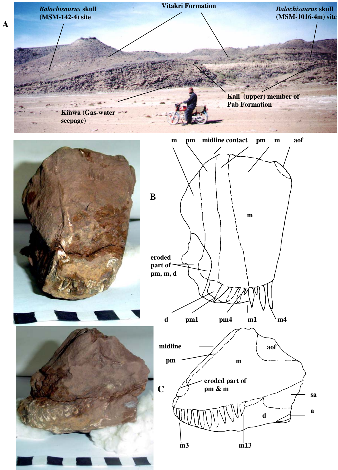
Fig. 3. A, Kinwa locality showing the Balochisaurus skulls sites. B, Photograph and line drawings of skull (rostrum) articulated with mandible (MSM-142-4) of Balochisaurus . anterior view. C, left lateral view. Scale for B and C, each black digit is 1 centimeter (cm). Abbreviation; a, angular; aof, antorbital fenestra; d, dentary; m, maxilla; pm, premaxilla; sa, surangular. Arabic numerals following abbreviations refer to tooth position (e.g., pm 4).
