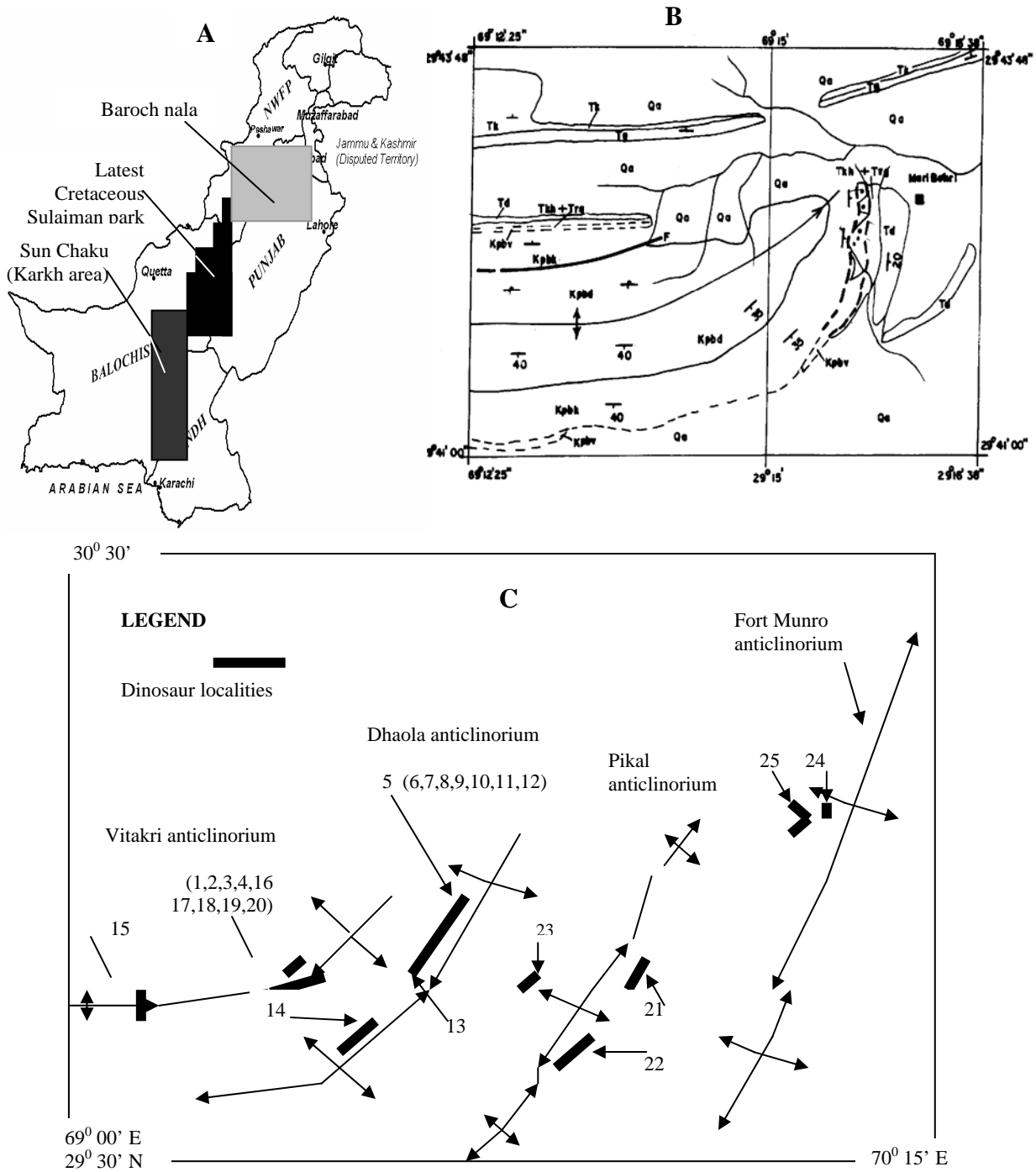
Fig. 1. A, light grey (upper) rectangle represents Kohat and Pothwar Basin, black (middle) rectangles represent the study area of Sulaiman Basin, medium grey (lower) rectangle represents Kirthar Basin of Pakistan. B, represents the map of Mari Bohri locality and fossil sites (dots), for symbols see Fig.2. C, represents the four major anticlinoria including the latest Cretaceous terrestrial fauna and their localities in Sulaiman Basin
