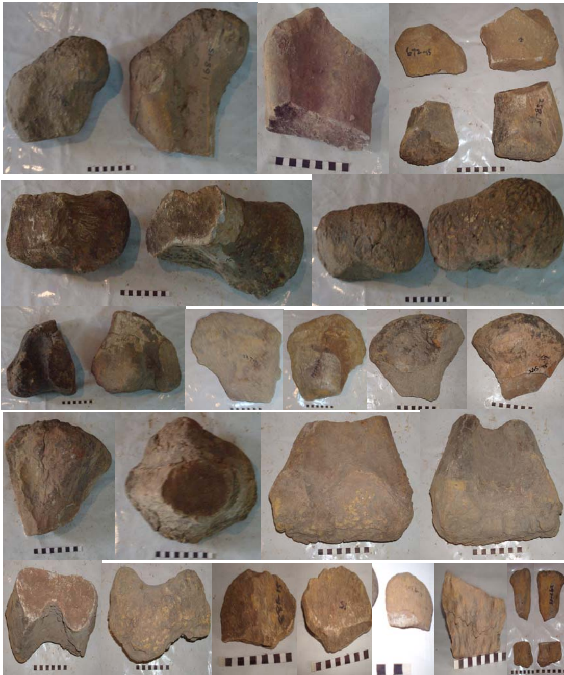
Fig. 6. First row, specimen nos started from left to right, MSM-167-15, MSM-168-15 and MSM-749-15, proximal left femora in posterior view; MSM-672-15 prox fibula (upper) and MSM-227-15 distal tibia (lower), MSM-717-15 proximal humerus (upper), MSM-258-15 distal humerus (lower); second row MSM-167-15 and MSM-168-15 proximal left femora in ventral and dorsal views; third row MSM-170-15 and MSM-173-15 distal femora; MSM-237-10 proximal humerus in two views, MSM-245-15 proximal humerus in two views; fourth row MSM-246-15 proximal left tibia stocky in lateral and dorsal views, MSM-174-15 distal humerus in anterior and posterior views; fifth row MSM-174-15 distal humerus in dorsal and ventral views, MSM-881-15 cervical rib in two views, MSM-1056-15 possibly distal rib, MSM-675-15 anterior sternal, MSM-297-15 proximal metacarpal (upper), MSM-750-15 distal metacarpal (lower) in two views. Scale, each black digit is 1 cm.
