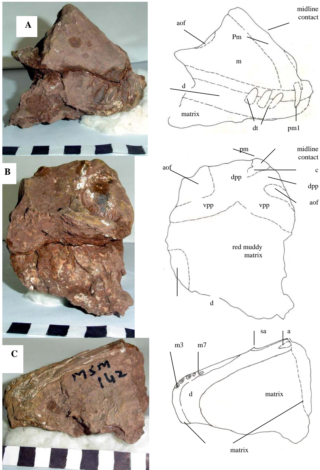
Fig. 4. Photographs and line drawings of skull (rostrum) articulated with mandible (MSM-142-4) of Balochisaurus , A, right lateral view; B, posterior view; C, ventral view. Scale, each black digit is 1cm. Abbreviations; a, angular; aof, antorbital fenestra; c, cavity; d, dentary; dpp, dorsal palatal process; dt, dentary teeth; m, maxilla; pm, premaxilla; sa, surangular; vpp, ventral palatal process. Arabic numerals following abbreviations refer to tooth position (e.g., pm 1).
